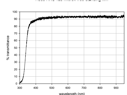
UV-vis of A535-AN-S film, 125 µm thickness
