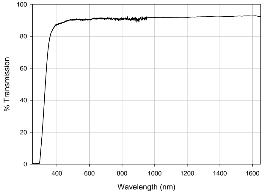
A535-AT 20 micron film between glass slides
