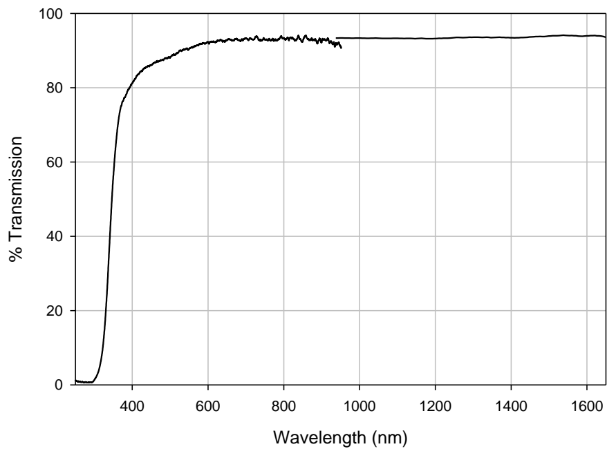
A535-A 20 micron cured adhesive film, glass substrates
